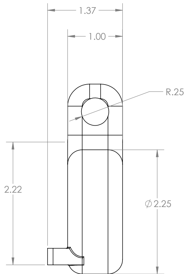
SIDE
