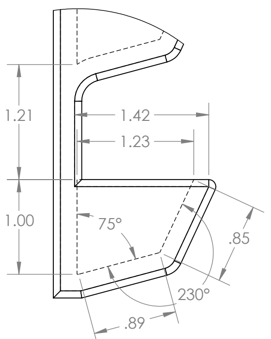
DETAIL F SCALE 1 : 1
