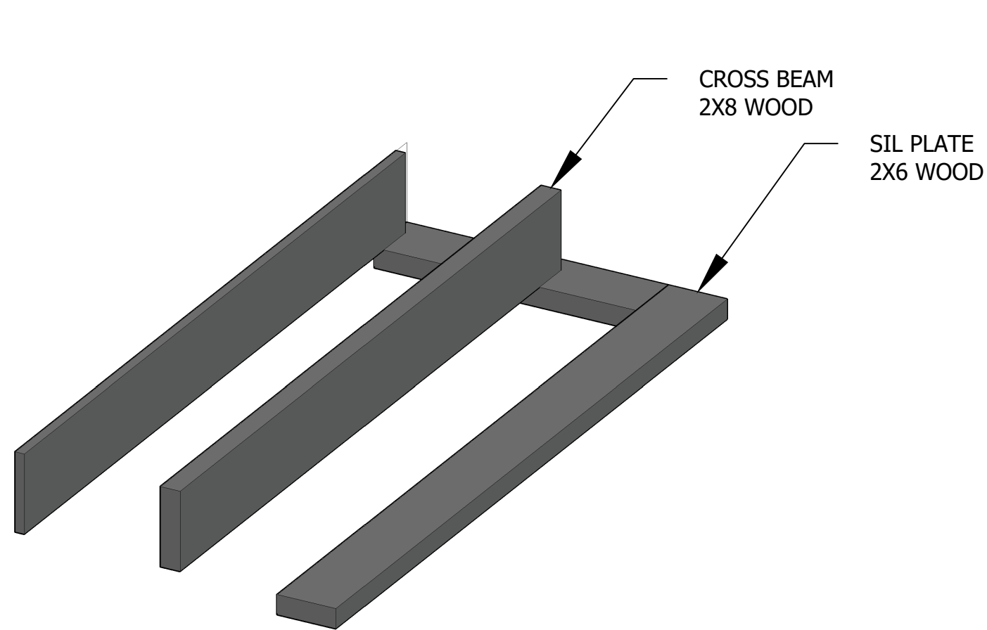
2 CORNER DETAIL VIEW SCALE: 3/8"=1' 0"
