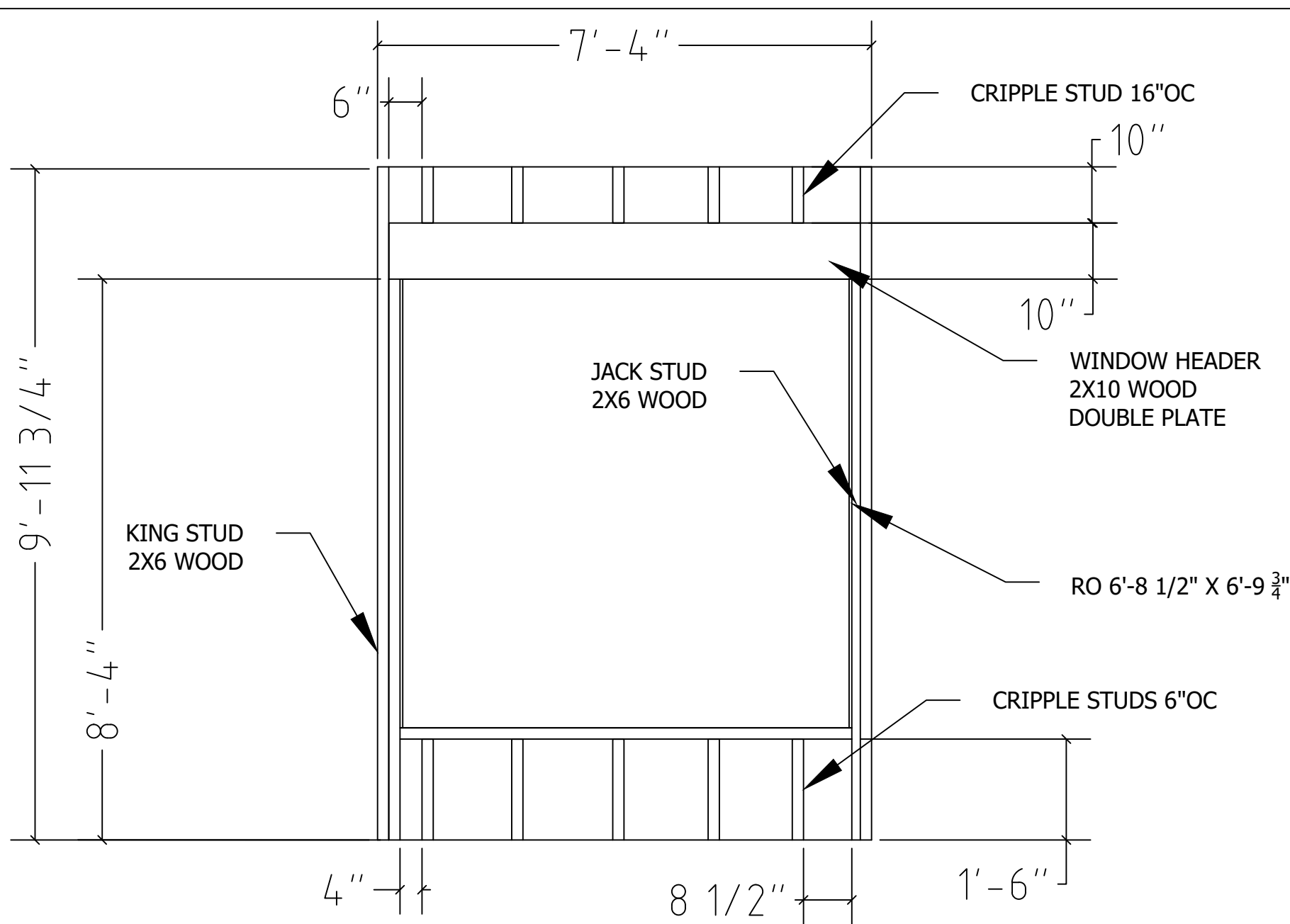
2 WINDOW DETAIL SCALE: 1/2"=1' 0"
