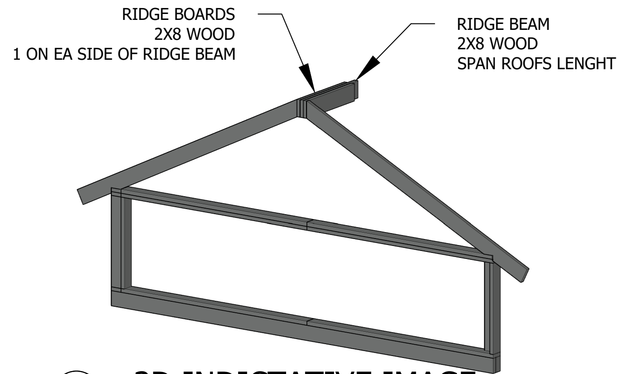
1-2 3D INDICATIVE IMAGE SCALE: 1/4"=1' 0"
