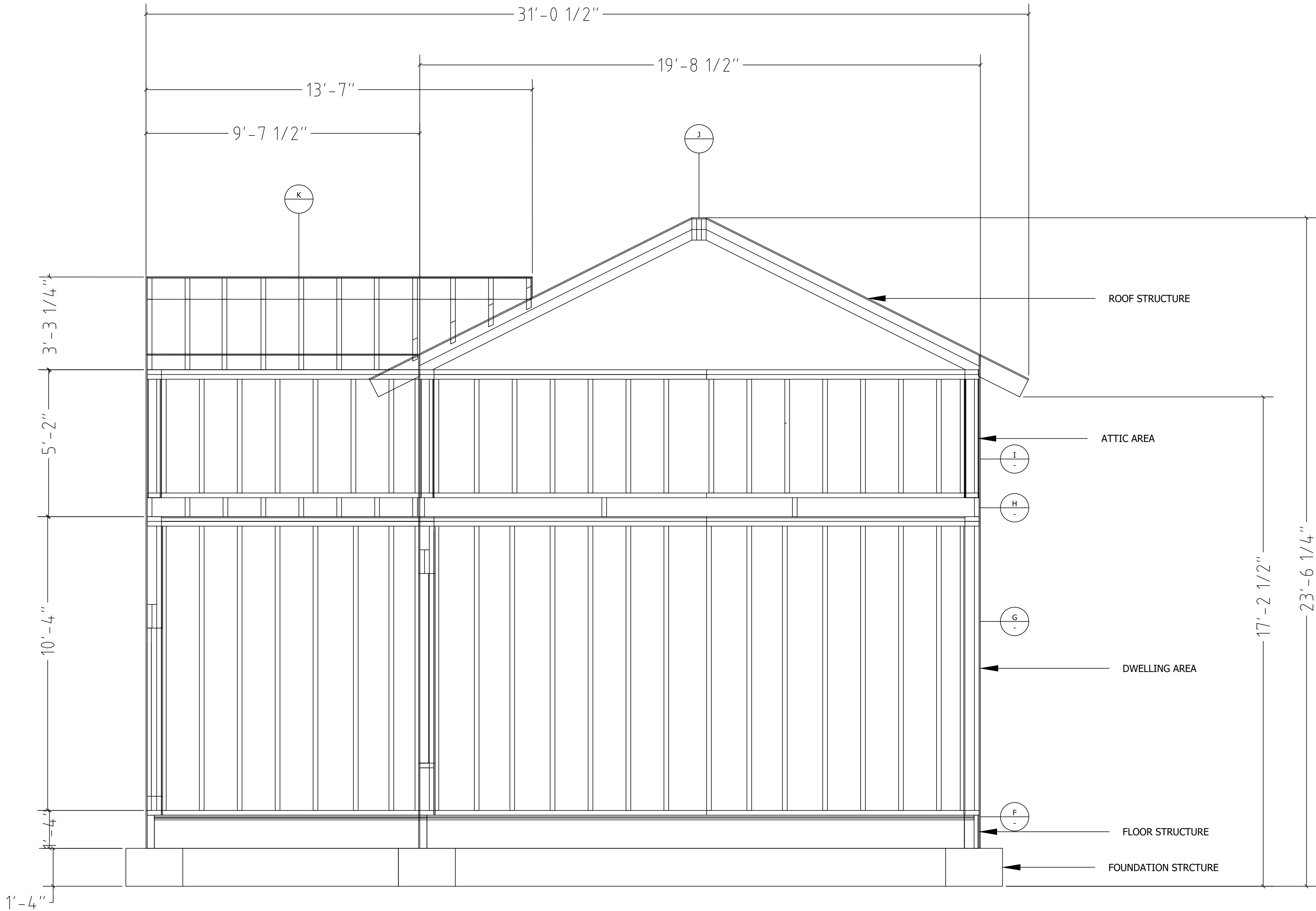
ELEVATION VIEW SCALE: 1/2"=1' 0"
