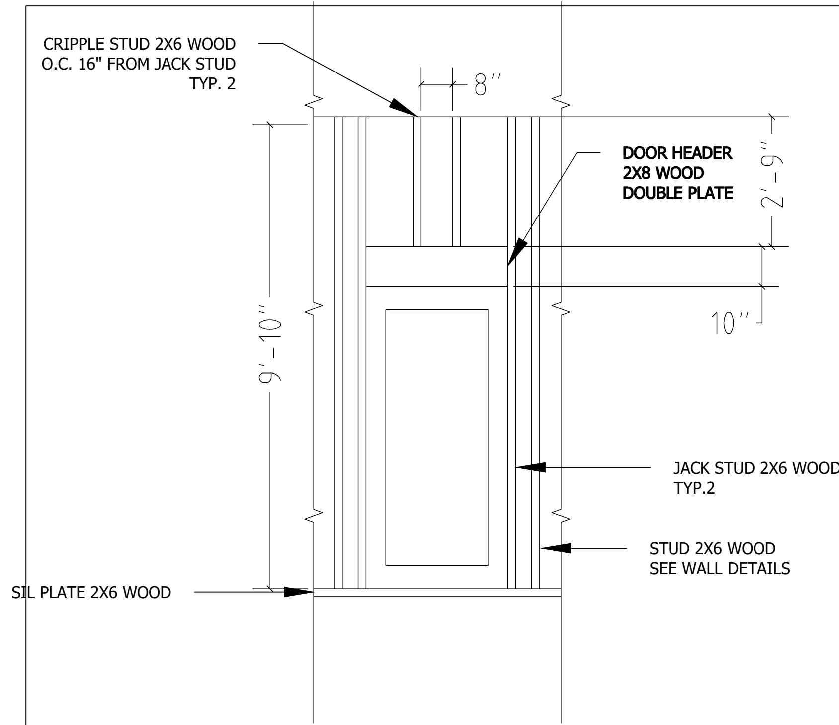
1 DOOR DETAIL SCALE: 1/2"=1' 0"
