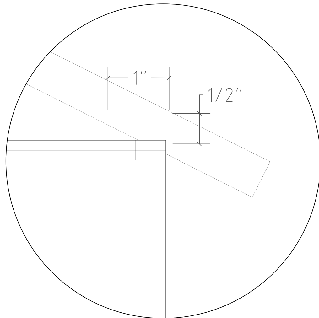
1-4 RAFTER NOTCH CUT
